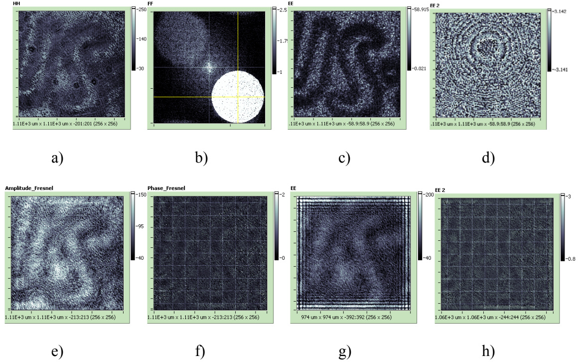
Figure 2.5. Holography of a US Coin. The image area is 1110 \times 1110 \mu m^2 ( 256 \times 256 pixels) and the image is at z = 198 \mu m from the hologram, \lambda = 0.575 \mu m , a = 1110 \mu m , N=256 pixels: (a) hologram; (b) angular spectrum; (c) amplitude and (d) phase images by the angular spectrum method; (e) amplitude and (f) phase images at minimum reconstruction distance z_{\min} = \frac{a^2}{N\lambda} = 8370 \mu m by the Fresnel transform method; (g) amplitude and (h) phase images at the reconstruction distance z = 8000 \mu m ( z < z_{\min} ) by the Fresnel transform method.
