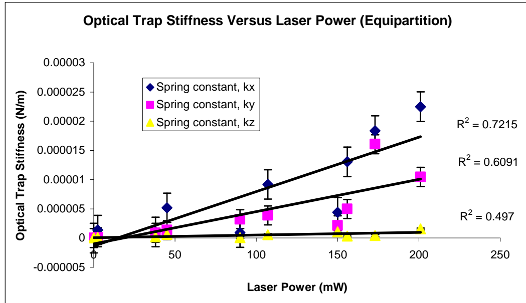
Figure. 7.10. Equipartition Calibration Method. Spring constant as a function of the laser beam power. R^2 (=Regression Sum Squares / Total Sum Squares) represents a figure of merit of curve fitting; R^2 = 1 means a perfect fit.
